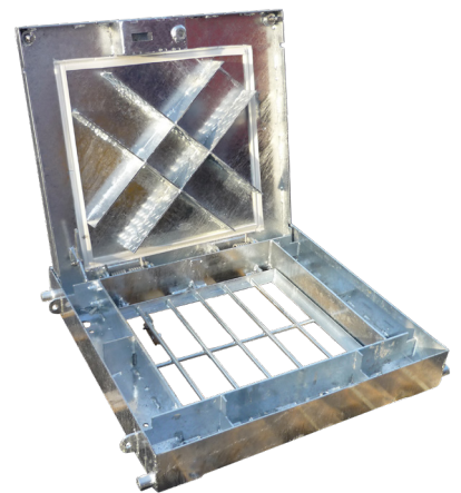
LPCB Range LPS 1175 SR3/4 High Security Flush & Upstand Units
